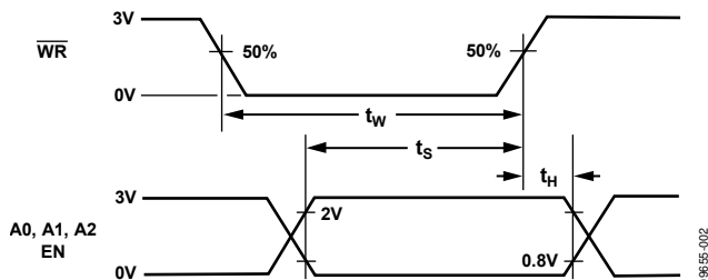
Figure 2. Timing Sequence for Latching the Switch Address and Enable Inputs
