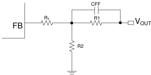
Figure 3. Feedback Divider Network
