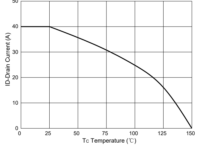
Fig. 10 - Drain Current
