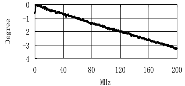
Phase Balance
