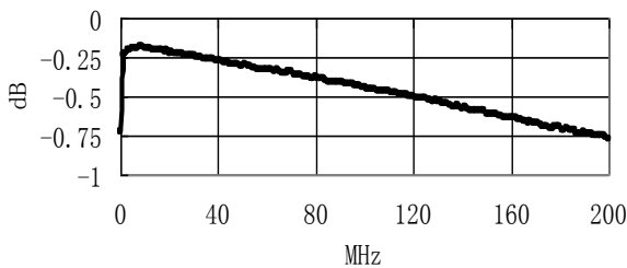
Insertion Loss
