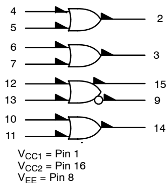
Figure 1. Logic Diagram
