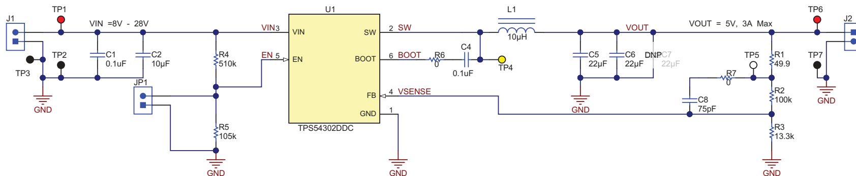
Figure 4-1. TPS54302EVM-716 Schematic
