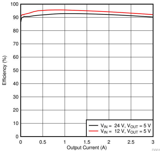
Figure 2-1. TPS54302EVM-716 Efficiency
