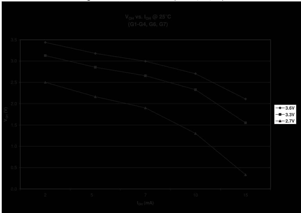
Figure 31. V_{OH} vs. I_{OH} @ 25°C (G1-G4, G6, G7)
