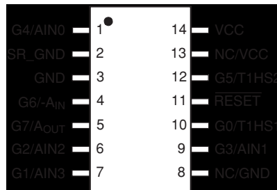
FMS7401L 14-Pin PDIP/SOIC/TSSOP
