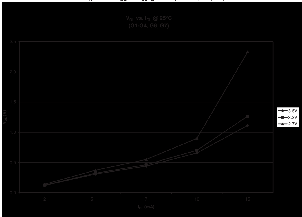
Figure 29. V_{OL} vs. I_{OL} @ 25°C (G1-G4, G6, G7)
