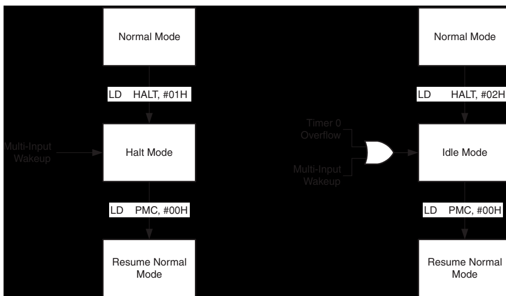
Figure 5. Recommended Halt/Idle Flow
