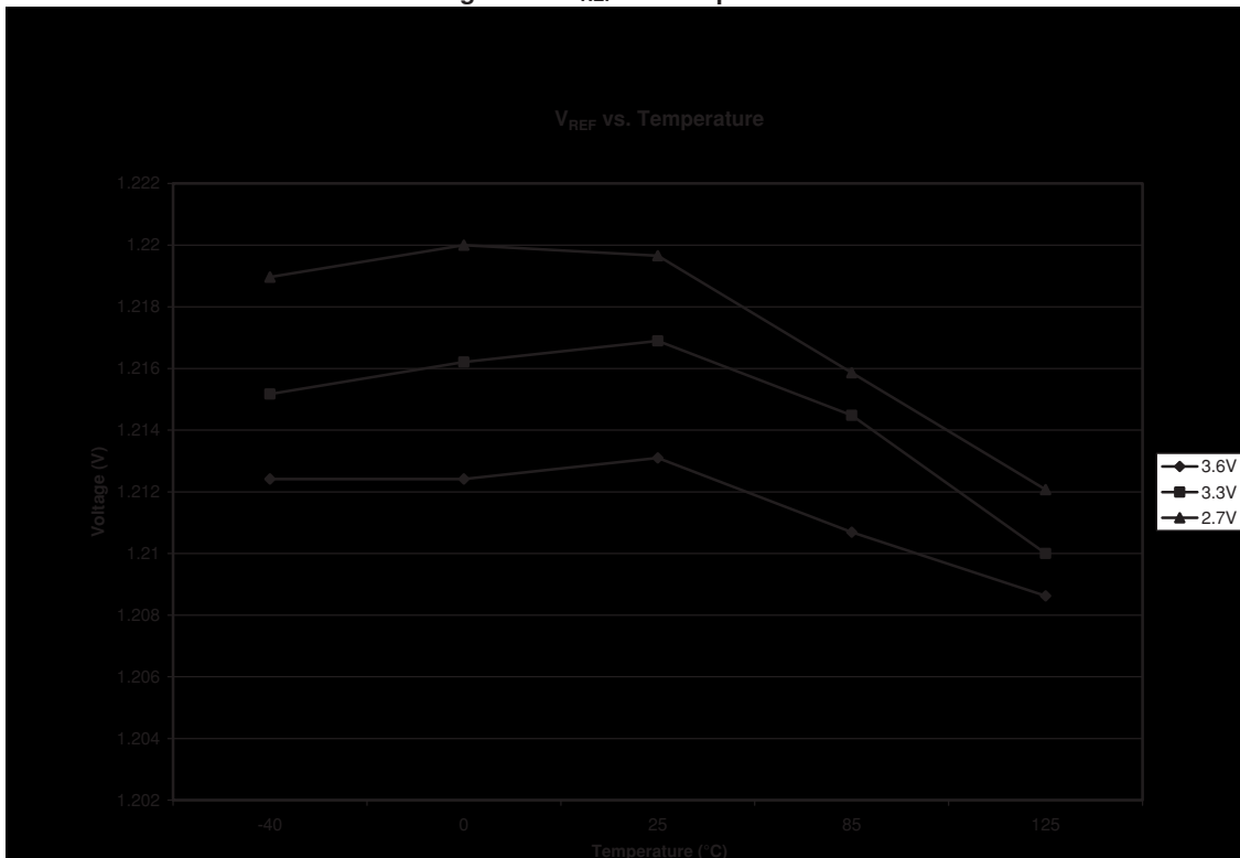
Figure 35. V REF vs. Temperature
