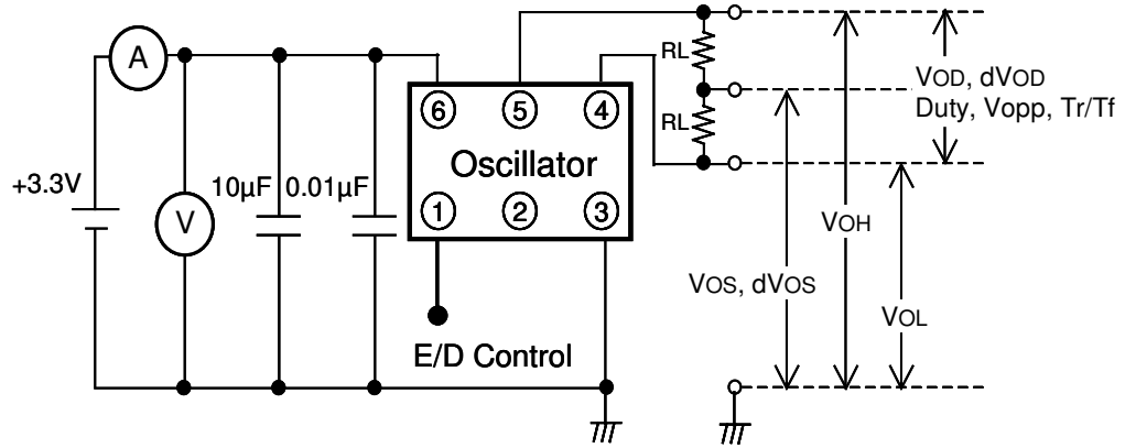
Fig.1 Test Circuit
