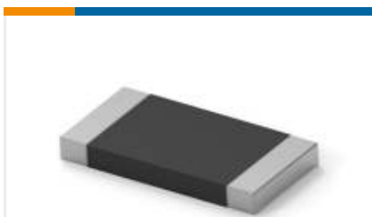
TE Part #7-2176421-9 TLRP 2512 2.0W R012 1% 75PPM 4K RL
