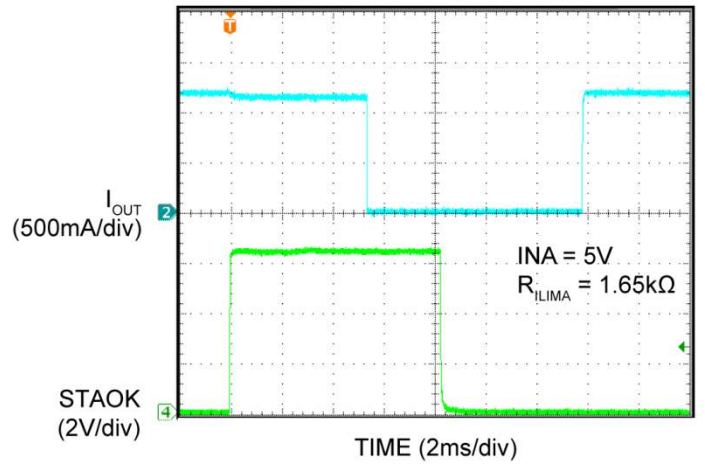
Current-Limit Response
