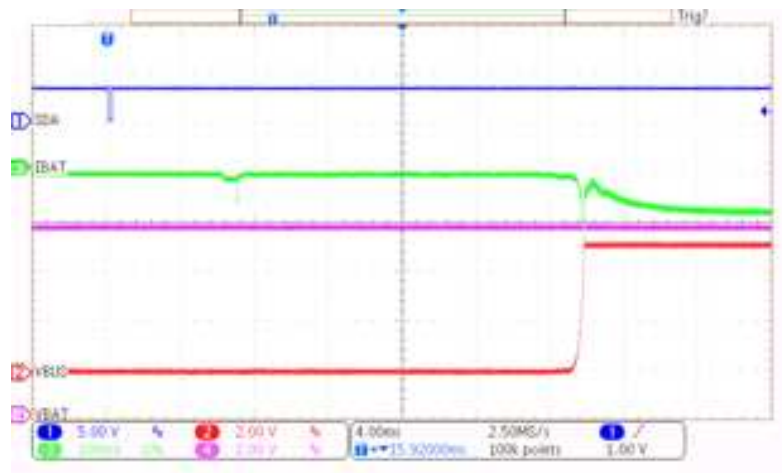
Figure 4. OTG Mode Startup
