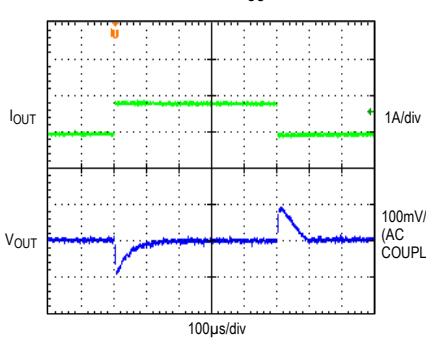
LOAD CURRENT TRANSIENT RESPONSE V_{IN} = 24V, V_{OUT} = 5V, I_{OUT} = 0.05A - 0.85A, MODE = VCC
