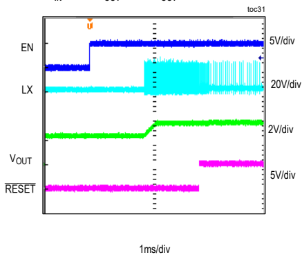
STARTUP WITH 2.5V PREBIAS V_{IN} = 24V, V_{OUT} = 3.3V, I_{OUT} = 0A, MODE = OPEN
