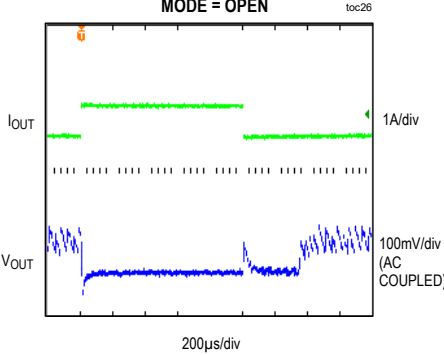
LOAD CURRENT TRANSIENT RESPONSE V_{IN} = 24V, V_{OUT} = 5V, I_{OUT} = 0.05A - 0.85A, MODE = OPEN
