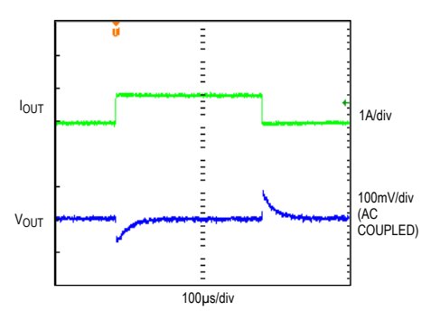
LOAD CURRENT TRANSIENT RESPONSE V_{IN} = 24V, V_{OUT} = 5V, I_{OUT} = 0.05A - 0.85A, MODE = SGND
