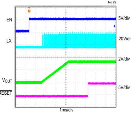
STARTUP THROUGH ENABLE V_{IN} = 24V, V_{OUT} = 3.3V, I_{OUT} = 0A, MODE = SGND
