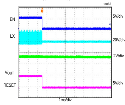
SHUTDOWN THROUGH ENABLE V_{IN} = 24V, V_{OUT} = 3.3V, I_{OUT} = 0A, MODE = SGND
