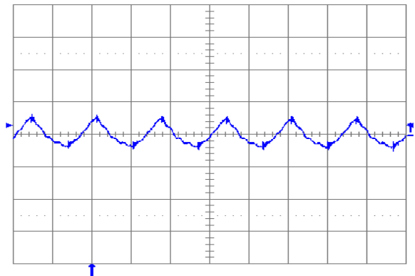
Fig. 5.0V.6: Output voltage ripple (20 mV/div.) at full rated load current into a resistive load with external capacitance 100\text{ }\mu\text{F} ceramic + 1\text{ }\mu\text{F} ceramic, and V_{in} = 12\text{ V} for V_{out} = 5.0\text{ V} . Time scale: 2 \mu\text{s} /div.
