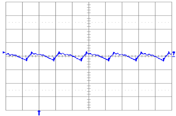
Fig. 2.0V.6: Output voltage ripple (20 mV/div.) at full rated load current into a resistive load with external capacitance 100\text{ }\mu\text{F} ceramic + 1\text{ }\mu\text{F} ceramic, and V_{in} = 12\text{ V} for V_{out} = 2.0\text{ V} . Time scale: 2 \mu\text{s} /div.
