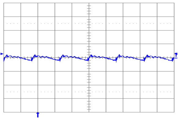
Fig. 1.2V.6: Output voltage ripple (20 mV/div.) at full rated load current into a resistive load with external capacitance 100\text{ }\mu\text{F} ceramic + 1\text{ }\mu\text{F} ceramic, and V_{in} = 12\text{ V} for V_{out} = 1.2\text{ V} . Time scale: 2 μs/div.
