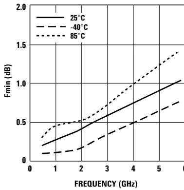
Figure 22. Fmin vs. Frequency and Temperature at 2.7V, 10 mA.
