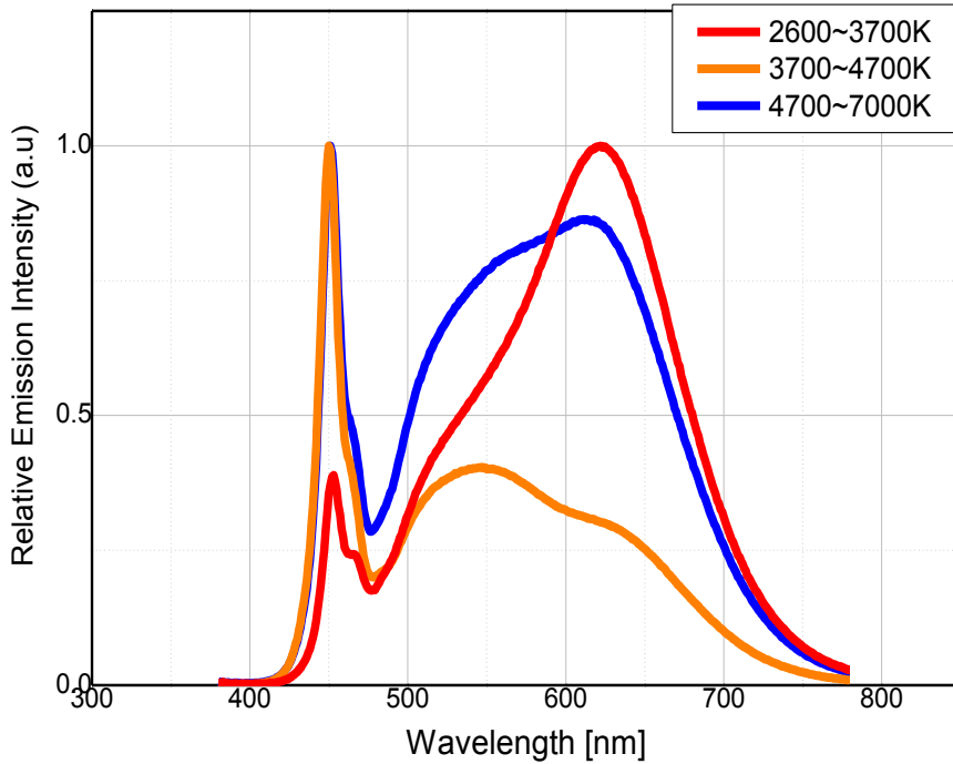
Fig 1. Color Spectrum, T_j = 25^\circ\text{C}
