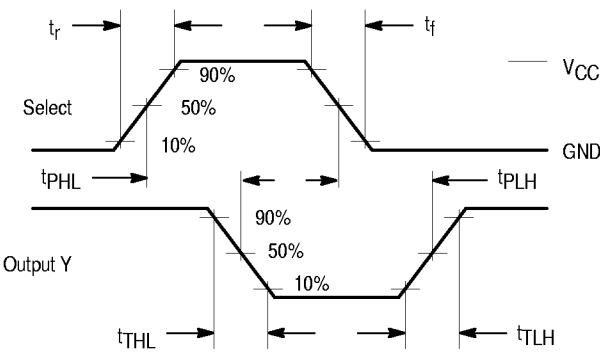
Figure 2. Y versus Select, Inverted
