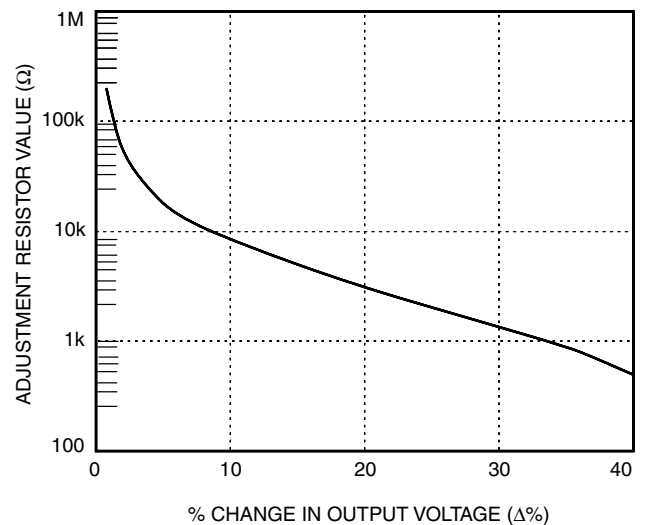
Figure 20. Resistor Selection for Decreased Output Voltage
