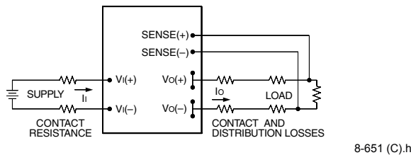
Figure 18. Effective Circuit Configuration for Single-Module Remote-Sense Operation
