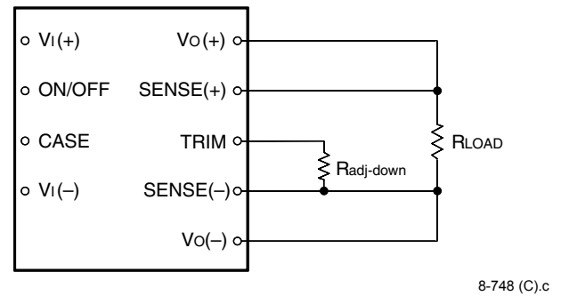
Figure 19. Circuit Configuration to Decrease Output Voltage
