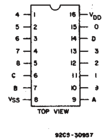
CD40147B TERMINAL ASSIGNMENT
