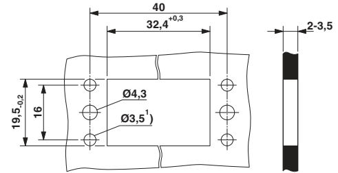
Dimensional drawing
