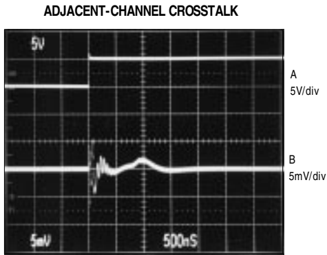
REF - = 4.096V, C L = 50pF, R L = 10kΩ A: DIGITAL INPUTS, DAC A, DATA BITS from ALL 0s to OAAAhex B: OUTPUT, DAC B
