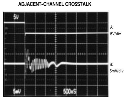
REF - = 4.096V, C L = 50pF, R L = 10kΩ A: DIGITAL INPUTS, DAC A, DATA BITS from OAAAhex to ALL 0s B: OUTPUT, DAC B
