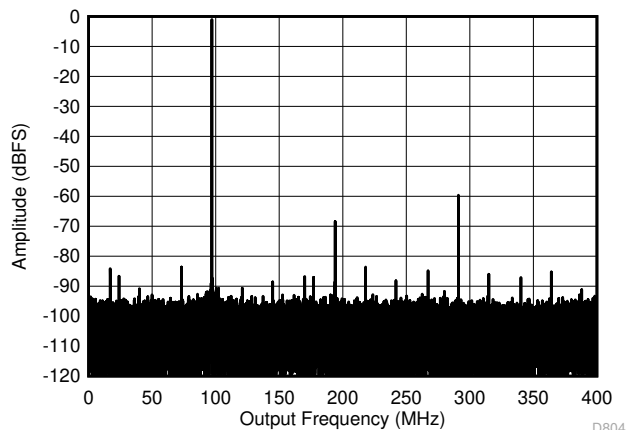
Figure 7-11. Single Tone FFT at 897 MHz and -1dBFS Low Power Mode
