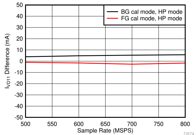
Figure 7-87. Quad Channel, I_{VD11} vs F_S over Modes
