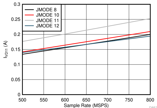
Figure 7-96. Dual Channel, I_{VD11} vs F_S for JMODES 8 - 12
