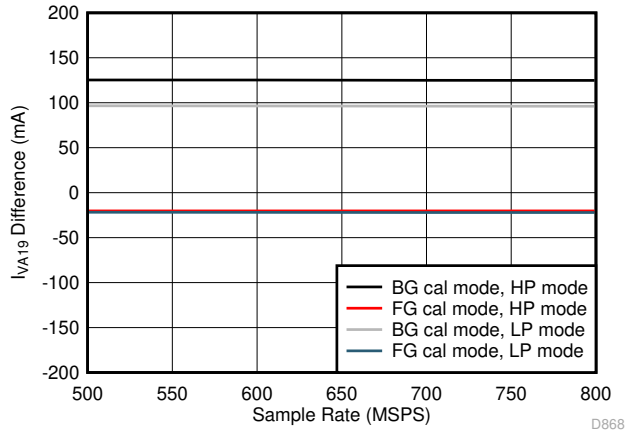
Figure 7-85. Quad Channel, I_{VA19} vs F_S over Modes
