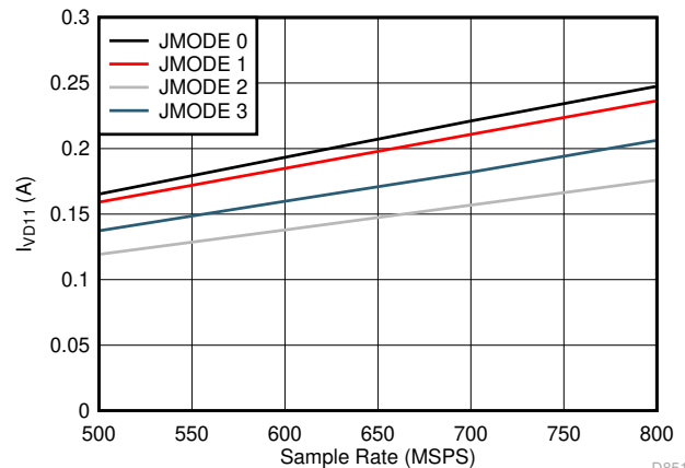
Figure 7-94. Dual Channel, I_{VD11} vs F_S for JMODES 0 - 3
