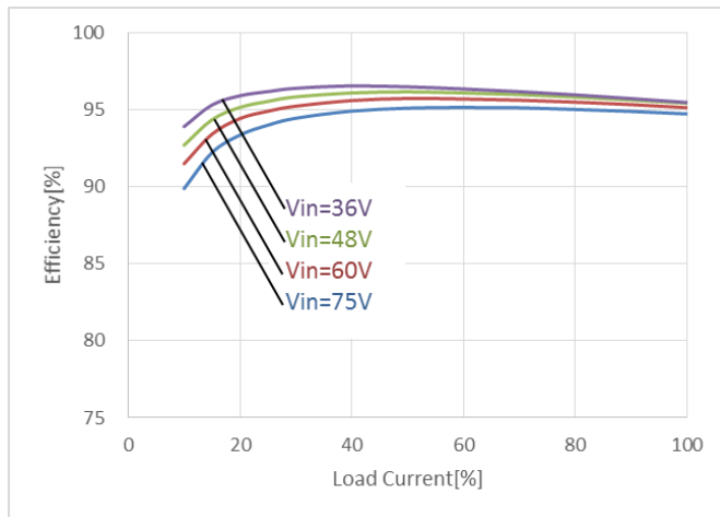
Effeciency vs, Line Voltage and Load Current @Ta = +25°C (100% : Vout12=10A,Vout5=1A)
