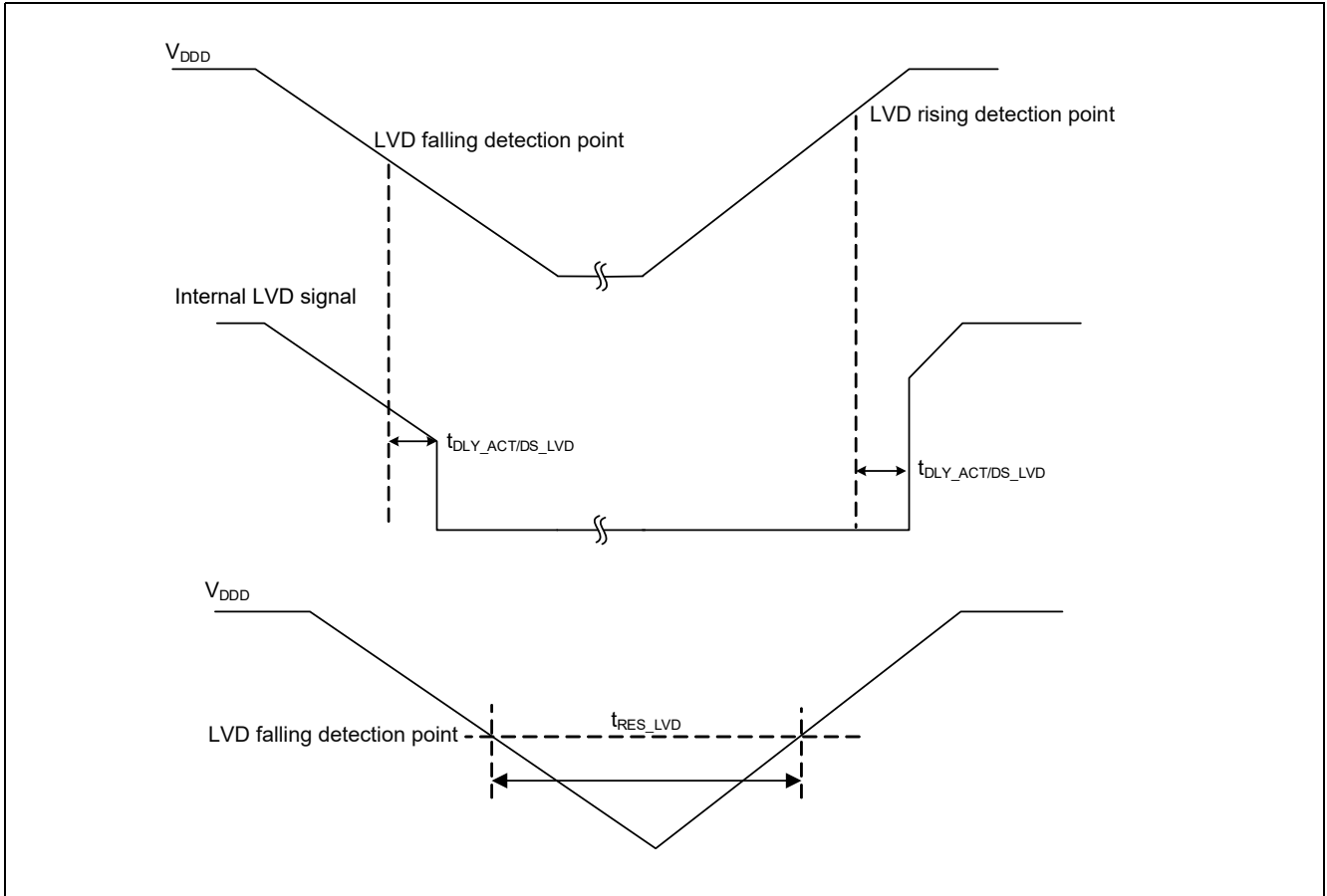
Figure 26-20 LVD specifications
