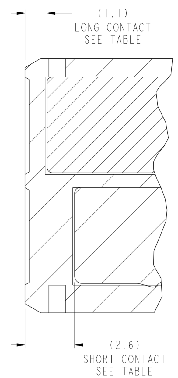
SECTION A-A SCALE 8:1
