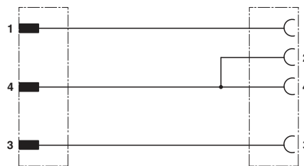
Contact assignment of M12 plugs / sockets bridged
