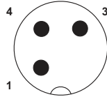
Pin assignment M12, 3-pos.
