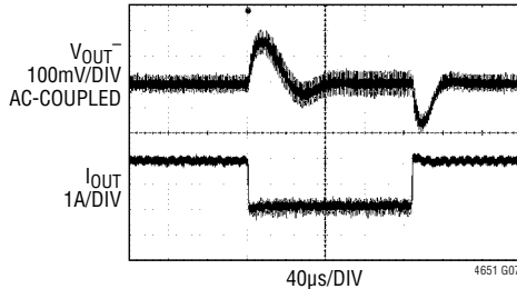
FIGURE 32 CIRCUIT, 24V IN , C_{IN} = C_{DGND} = C_D = 4.7\mu\text{F} , C_{OUT} = 47\mu\text{F} \times 2 , R_{ISET} = 665\text{k}\Omega , R_{ISET} = 100\text{k}\Omega , R_{PGDFB} = 36.5\text{k}\Omega , R_{EXTVCC} = 20\Omega , 1.8A TO 3.8A LOAD STEP AT 2A/ \mu\text{s}
