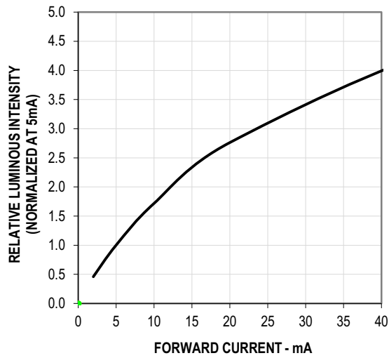
Figure 5: Intensity vs. Forward Current
