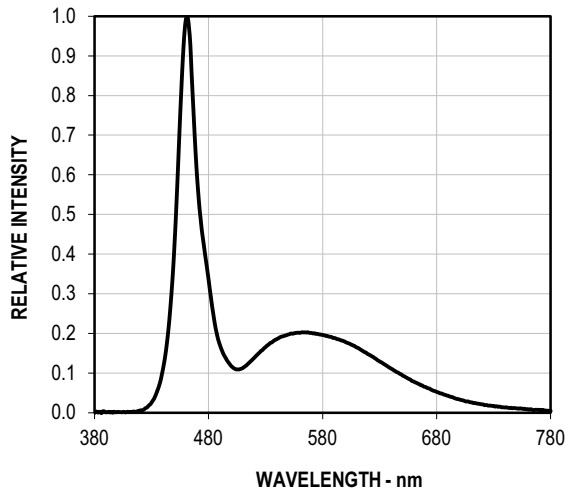
Figure 3: Intensity vs. Wavelength
