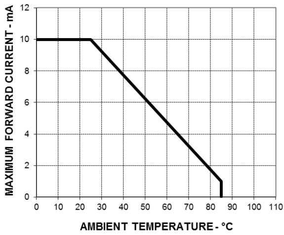
Figure 11: Forward Current vs. Temperature
