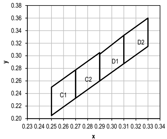
Figure 2: Chromaticity Coordinates Diagram
