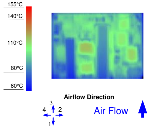
Figure 8. Thermal Image for Airflow Direction 3 (18A output, 55°C ambient, 200 LFM, typical Vin, open frame, unit soldered onto a fixture board)
