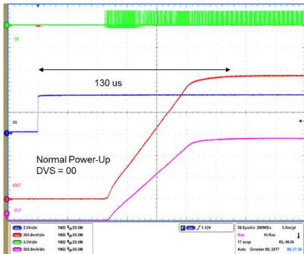
Figure 33. Normal Power Up, V_{OUT} = 1.15\text{ V} , DVS[1..0] = 00
