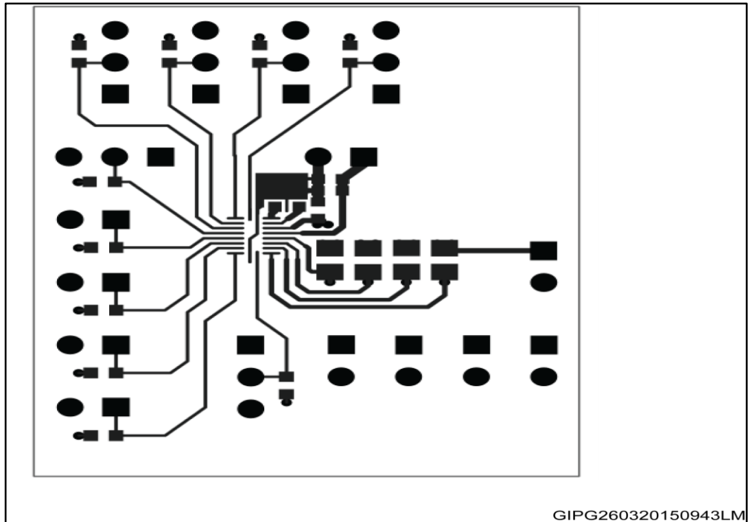
Figure 9: Top layer
