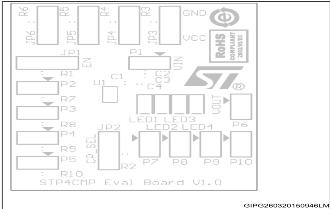
Figure 11: Top overlay
