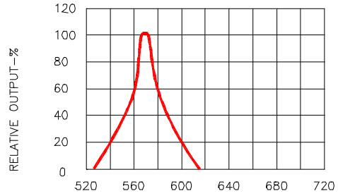
Fig.2 SPECTRAL RESPONSE
