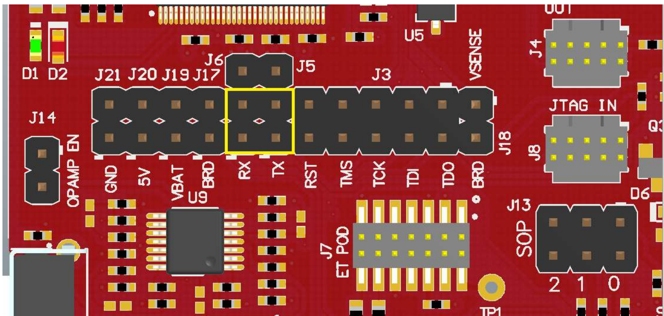
Figure 14. UART Routed to 20-Pin Header Connector
