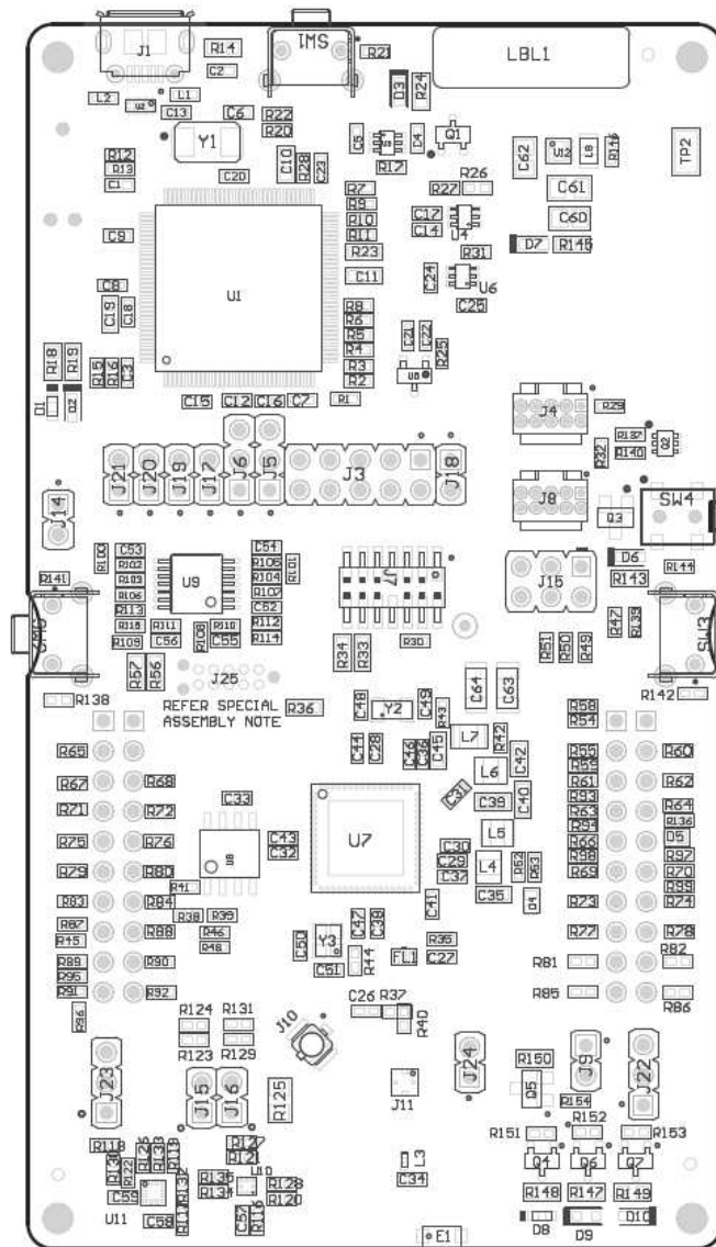
Figure 23. CC3220x LaunchPad Kit Top-Layer Assembly Drawing
