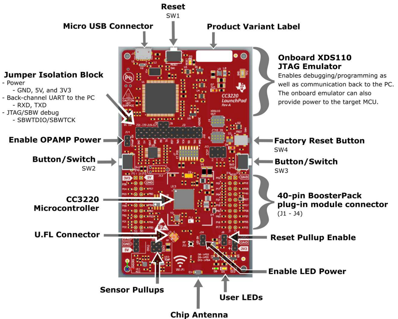
Figure 3. CC3220 LaunchPad Development Kit Overview
