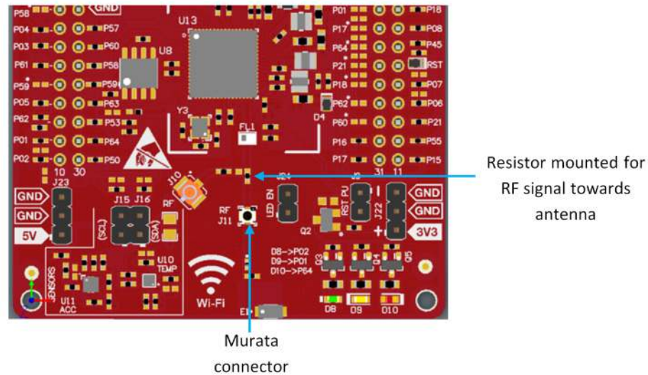
Figure 21. Using Onboard Antenna (Default Condition)
