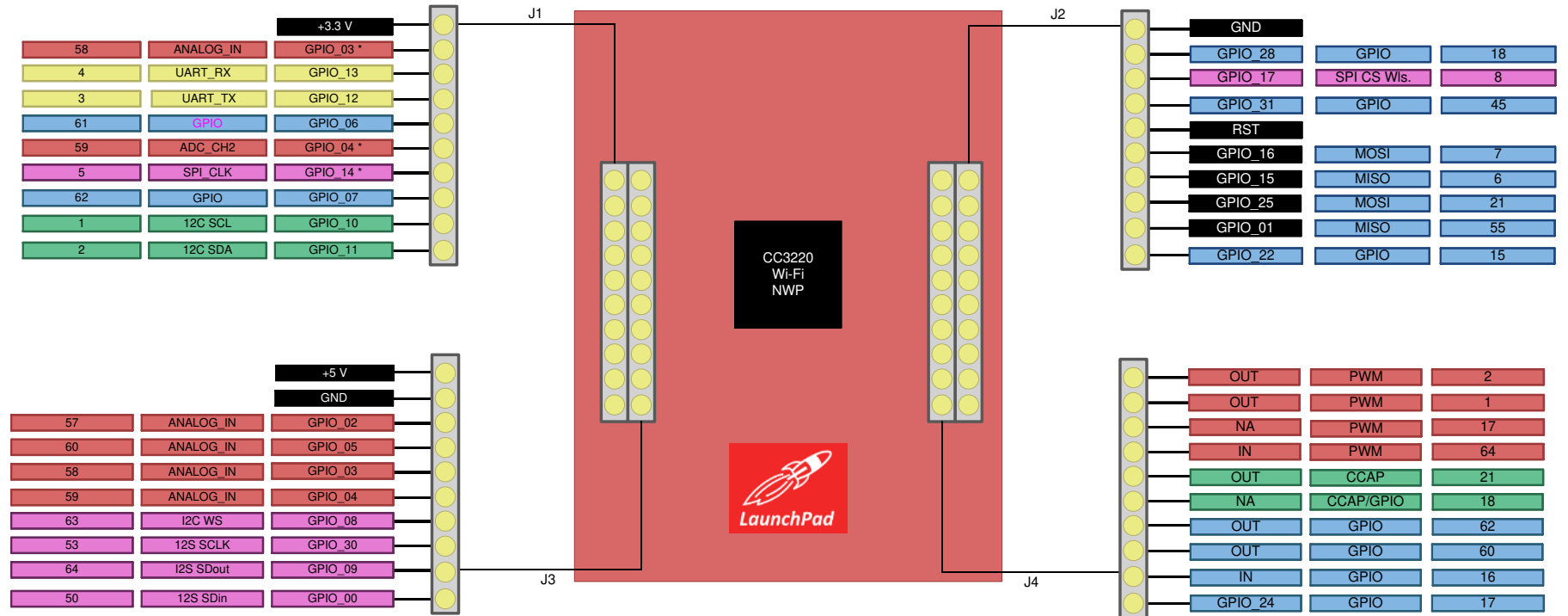
Figure 15. CC3220 BoosterPack Module Header Pin Assignments
