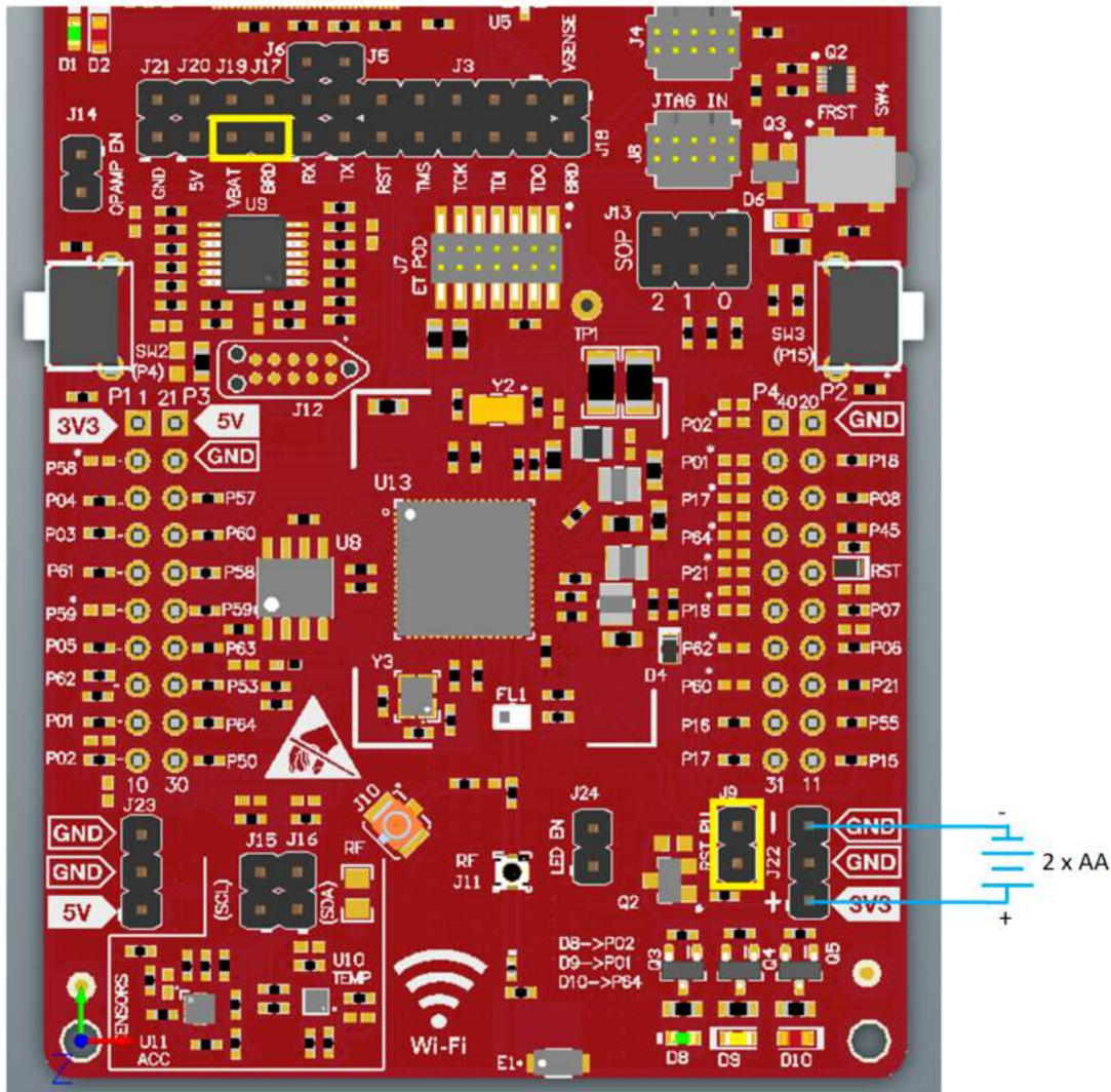
Figure 17. Powering the CC3220LP From Battery
