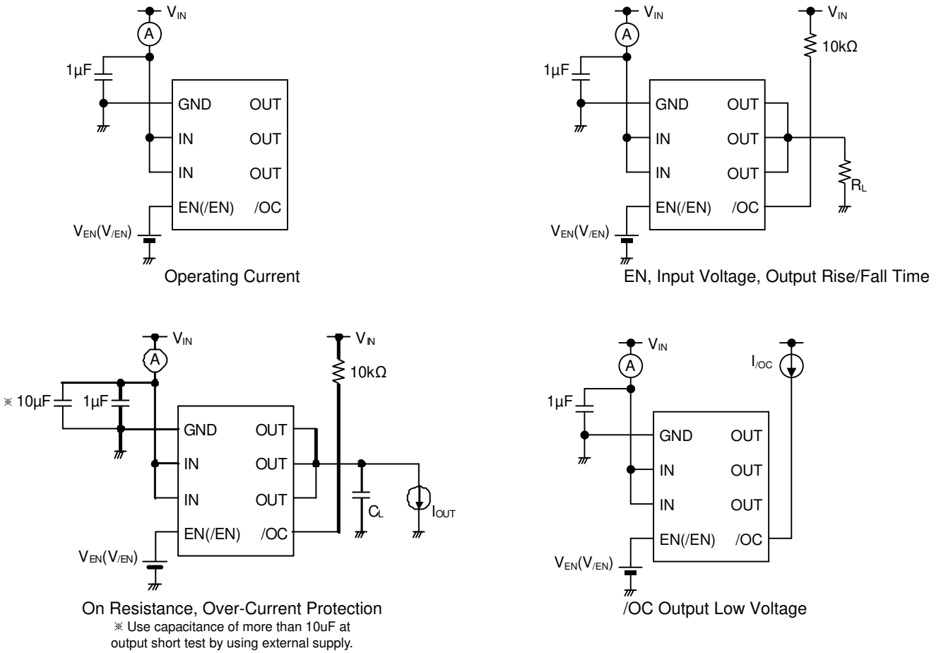
Figure 4. Measurement Circuit
