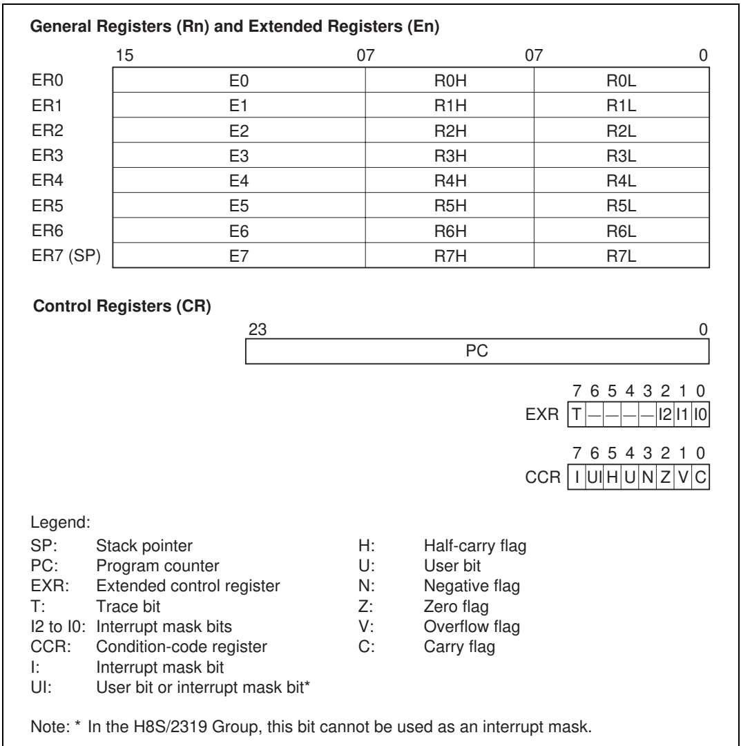
Figure 2.4 CPU Registers
