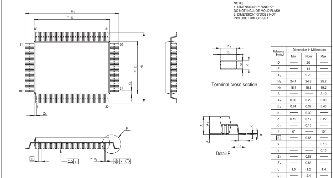
Figure F.3 FP-100A Package Dimensions
