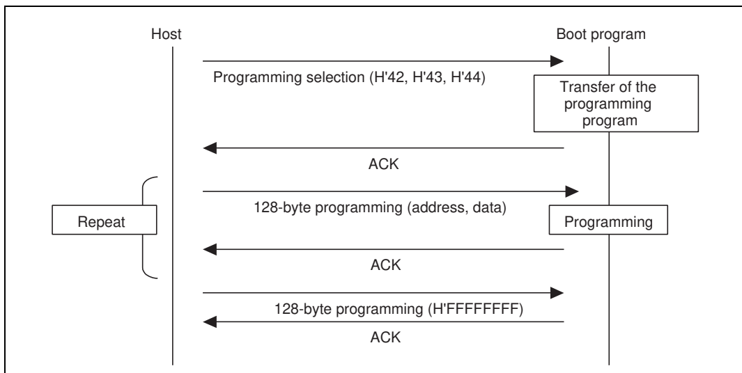
Figure 17.86 Programming Sequence
