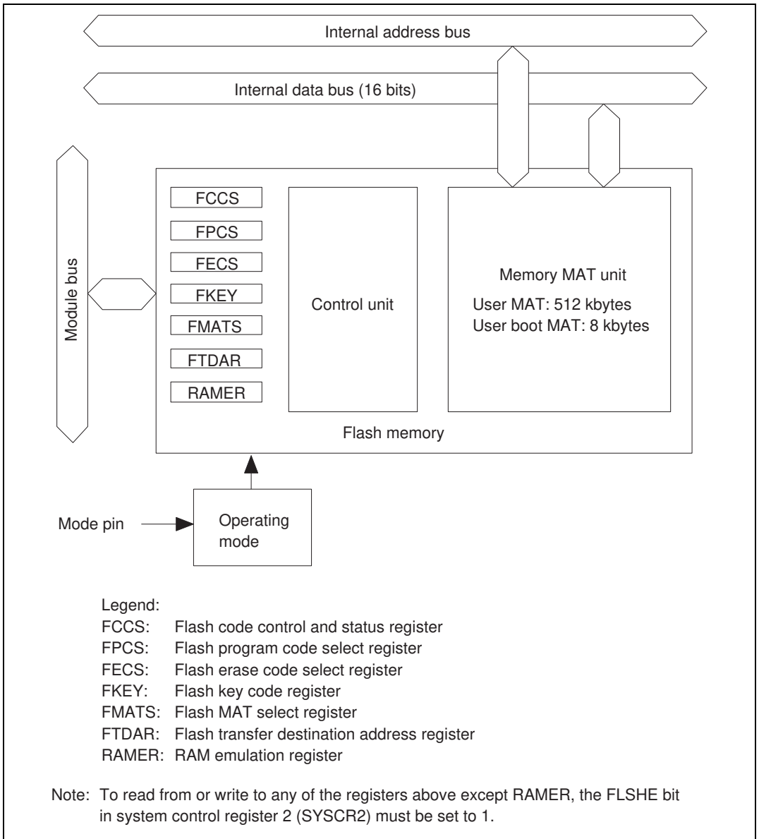
Figure 17.60 Block Diagram of Flash Memory
