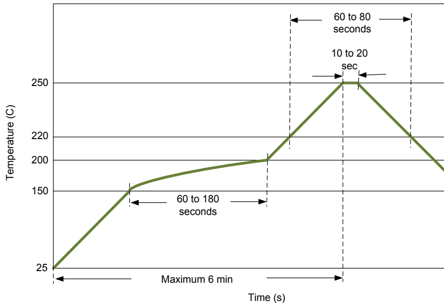
Figure 59: Reflow solder profile
