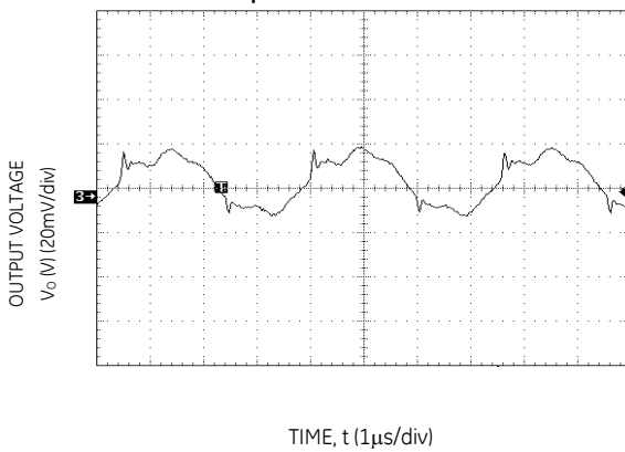
Figure 32. Typical Output Ripple and Noise (Vin =48Vdc, I_o = 12A).
