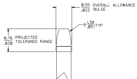
DETAIL F
