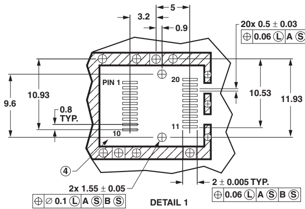
Figure 7b. SFP host board mechanical layout.
