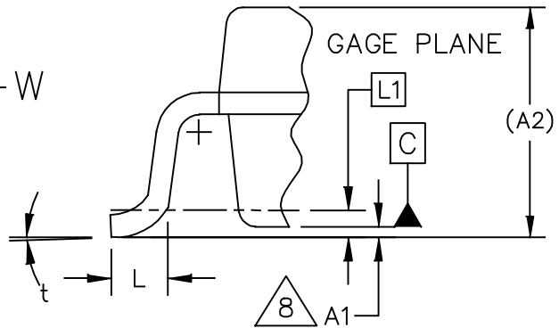
DETAIL "Y"
