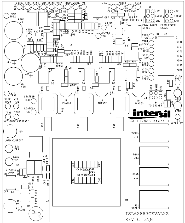
FIGURE 7. TOP SILKSCREEN
