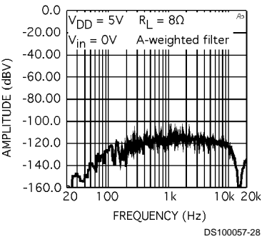
Power Amplifier Noise Floor
