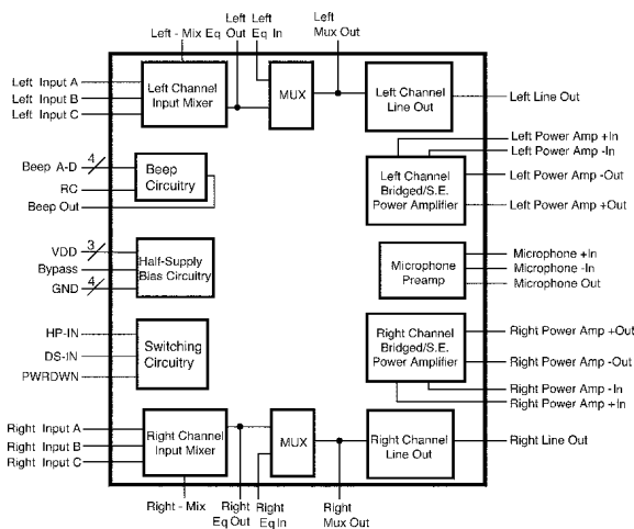
FIGURE 1. LM4831 Block Diagram
