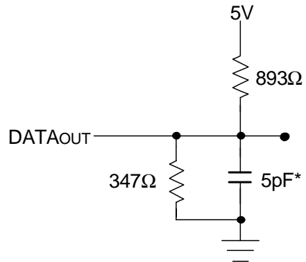
Figure 2. Output Test Load (for t LZ , t HZ , t wZ , t ov )
