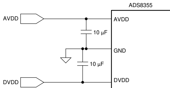
Figure 47. Power-Supply Decoupling
