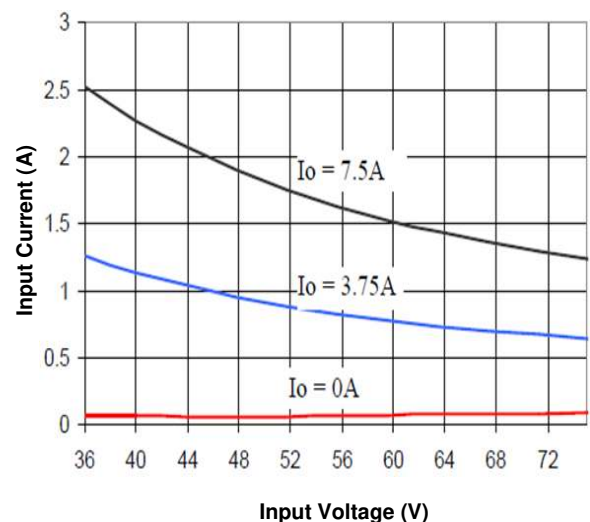
Figure 2. Input Characteristics
