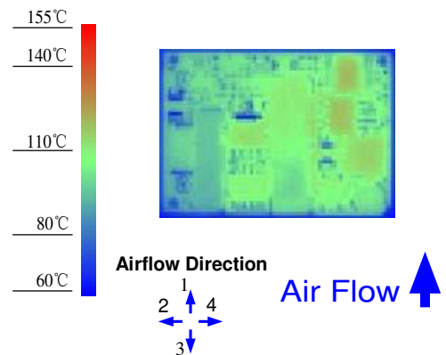
Figure 8. Thermal Image for Airflow Direction 1 (4.2A output, 70°C ambient, 0LFM, typical Vin, open frame, unit soldered onto a fixture board.)
