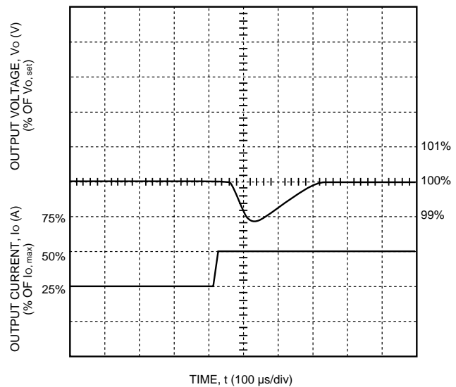
Figure 16. CW025 Triple-Output-Series Typical Output Voltage for a Step Load Change from 25% to 50% of Full Load on Output 1
