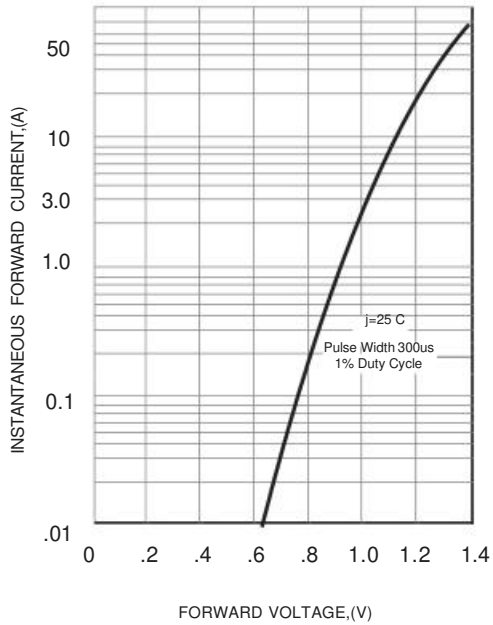
FIG.3-TYPICAL FORWARD CHARACTERISTICS
