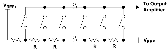
Figure 31. Resistor String
