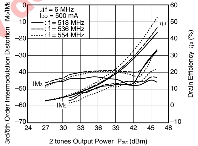
IM3/IM5, DRAIN EFFICIENCY vs. 2 TONES OUTPUT POWER
