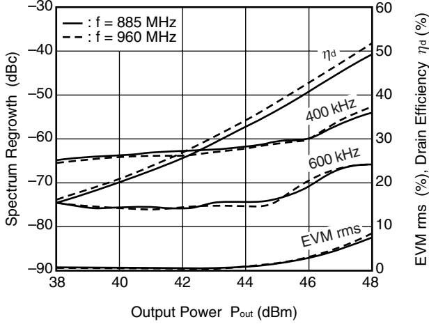
SPECTRUM REGROWTH, EVM rms, DRAIN EFFICIENCY vs. OUTPUT POWER
