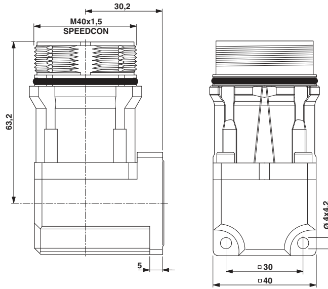
Dimensioned drawing
