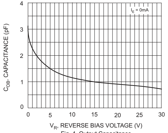
Fig. 4 Output Capacitance
